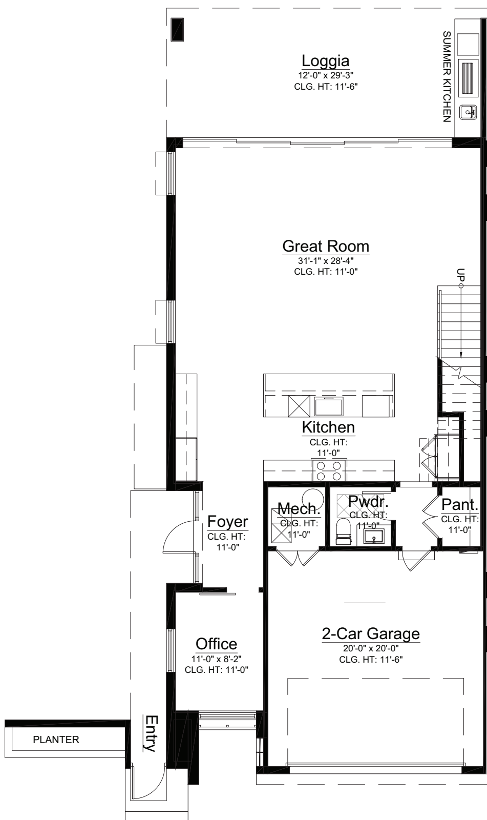
FIRST FLOOR
